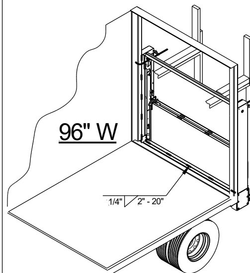
Traverse Welds
