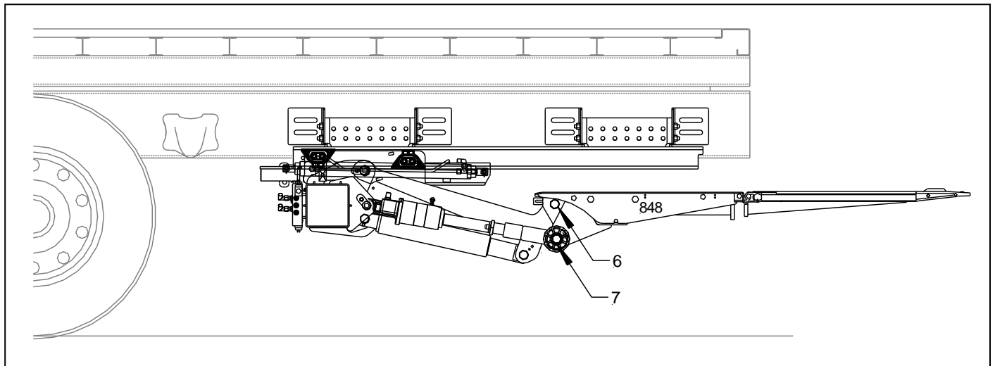
Figure 9 Platform Attachment
