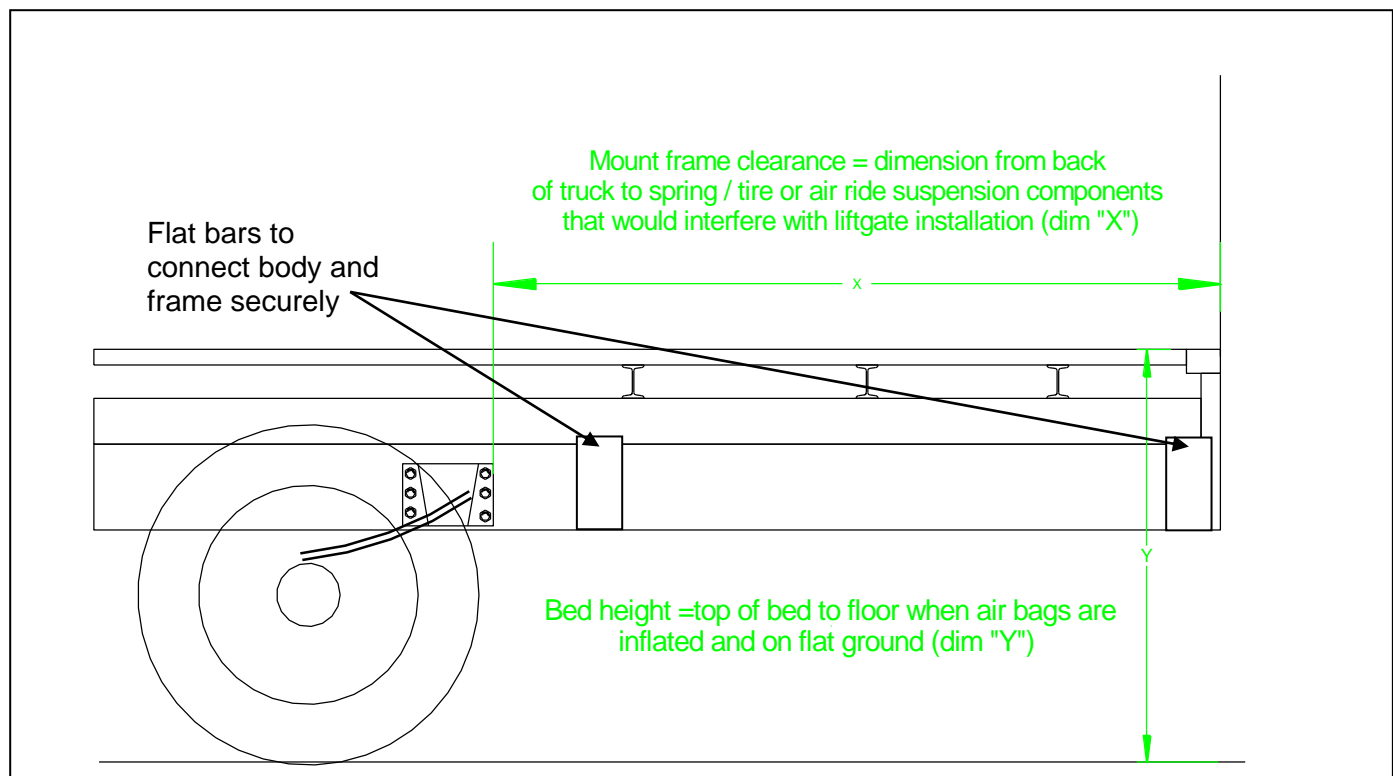
Figure 4 Mounting Clearance
