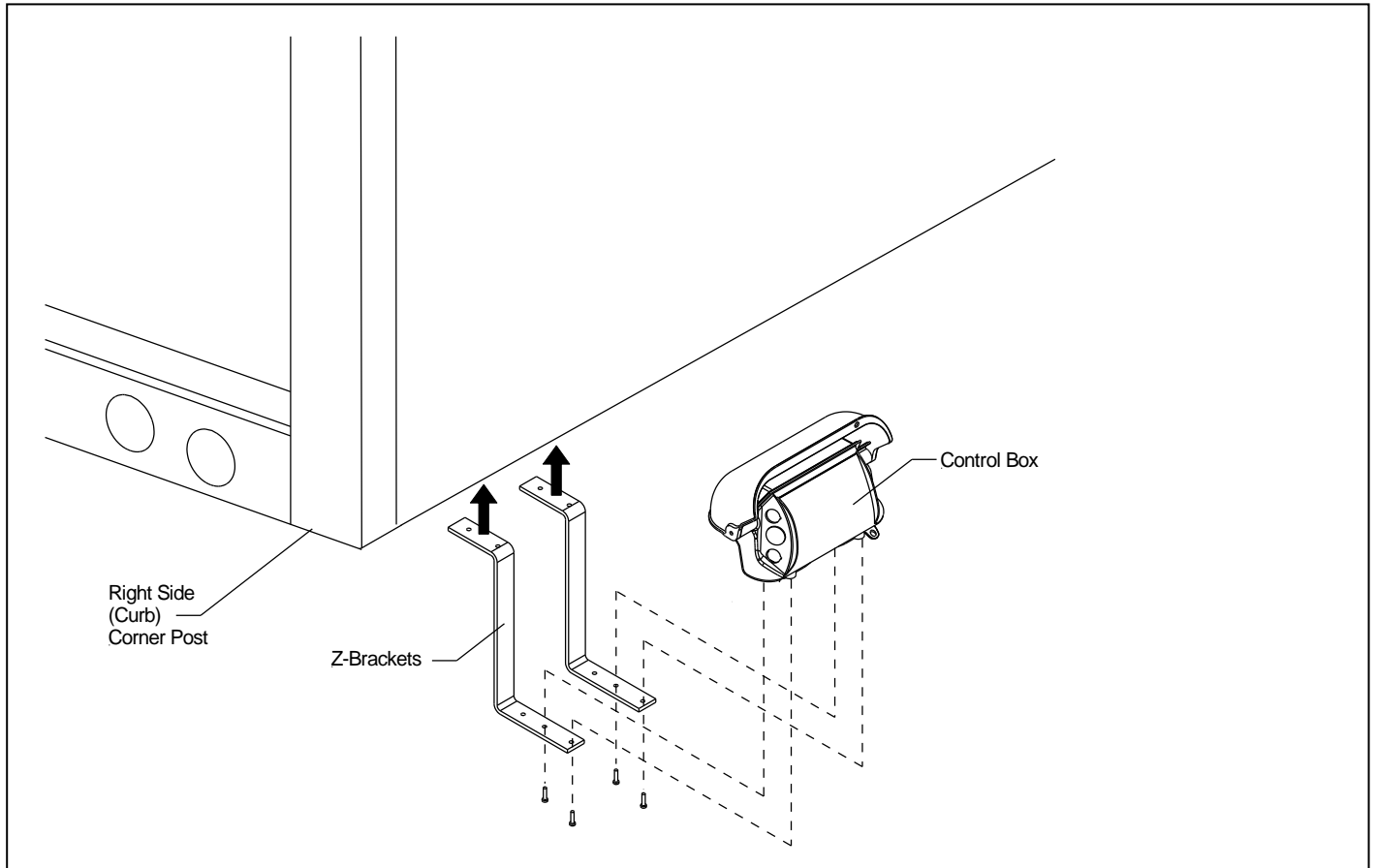
Figure 16 Control box placement
