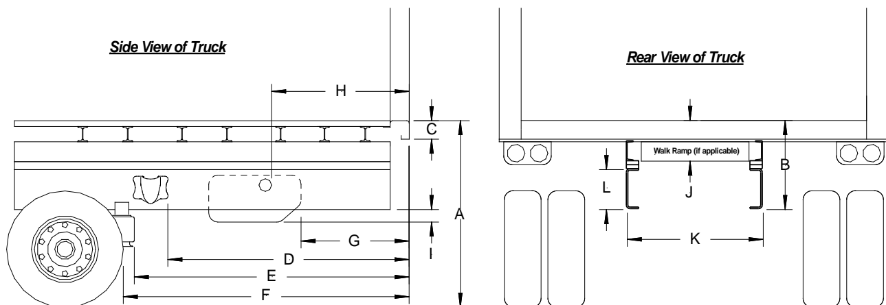
Figure 2 Truck dimension sheet
