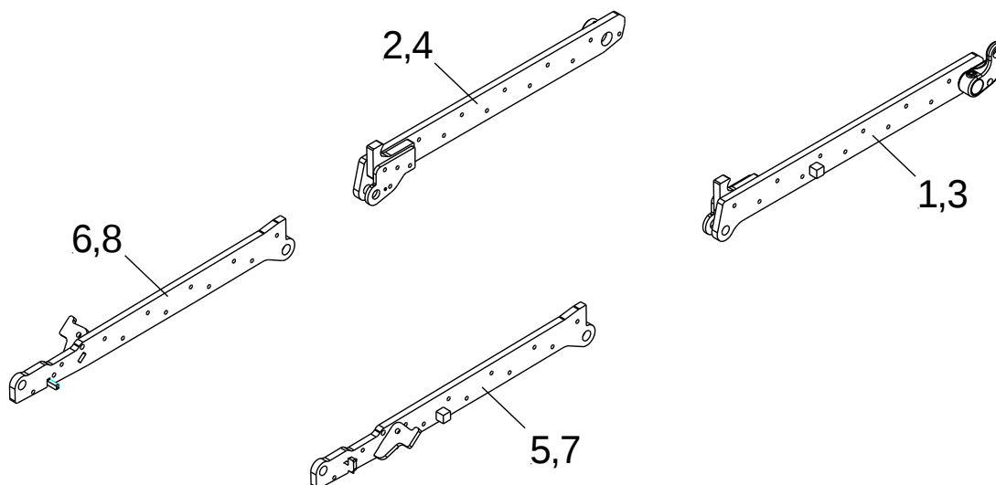
8 – ALUMINUM PLATFORM SIDE BAR ASSEMBLIES - MAIN SECTION
