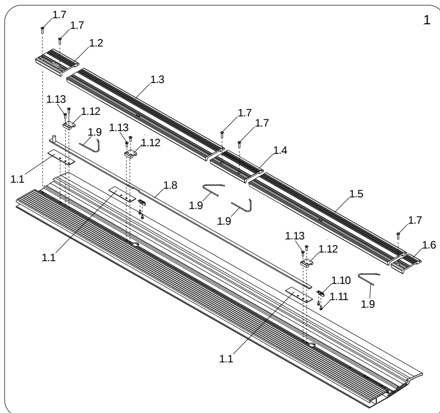
7.1 – CART STOPS ALUMINUM PLATFORMS
