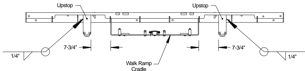
Front View of Bed Extension w/Walk Ramp Cradle and Upstops
