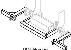
DOT Bumper Fig.4
