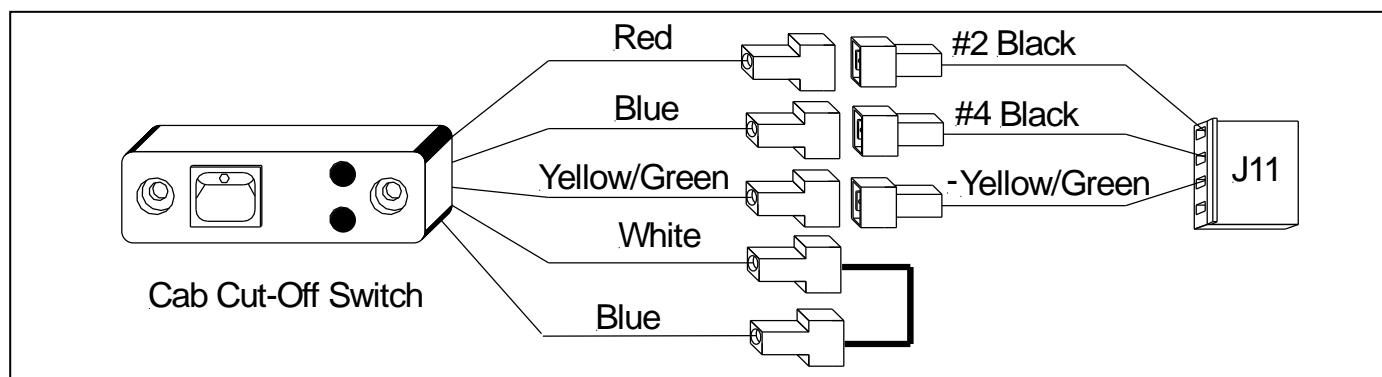
Figure 24 Cab Cut-off switch connection
