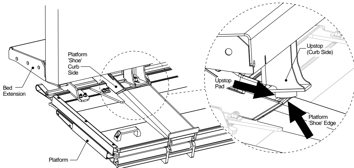
Bottom View of Upstop with Different Pad Positions
