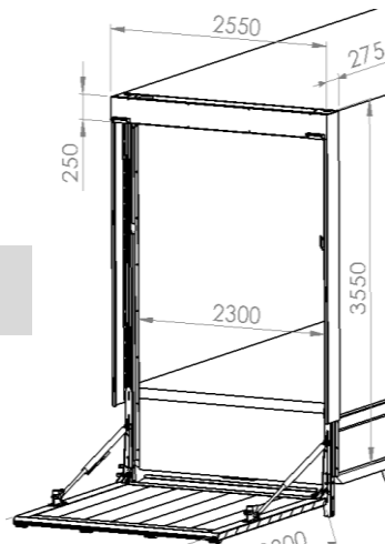
SCL1000/1500 Top A light car lift
