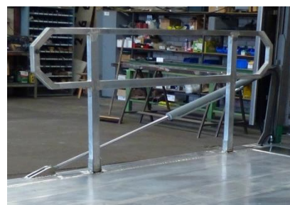
Safty rail (type 2)
